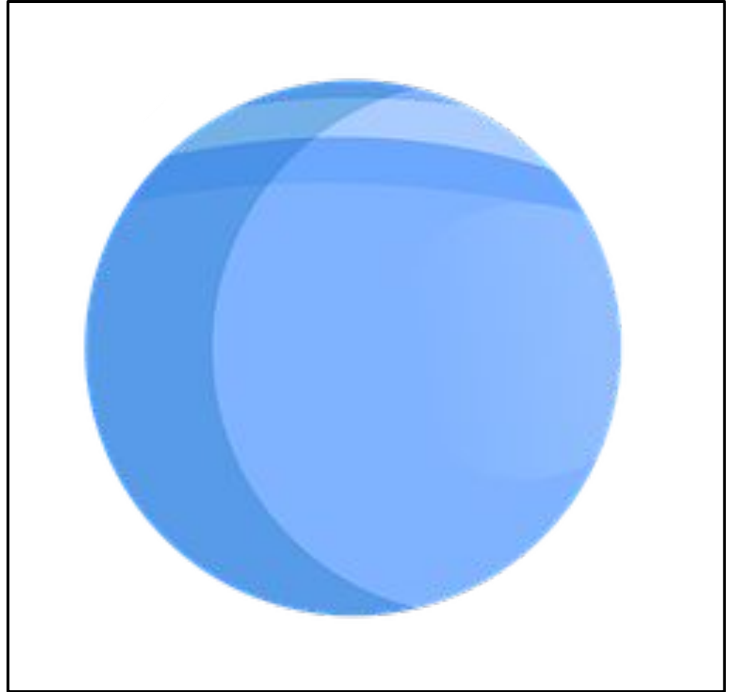
NEPTUNE
