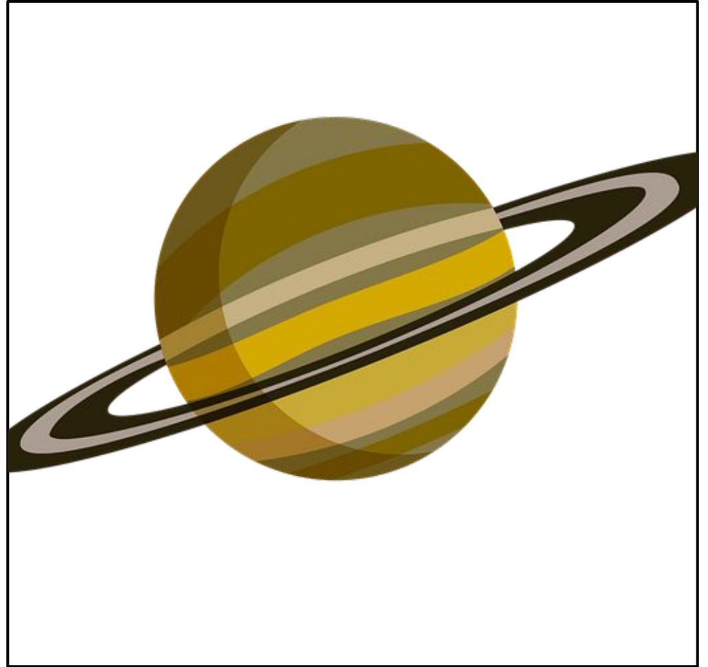
SATURNE
